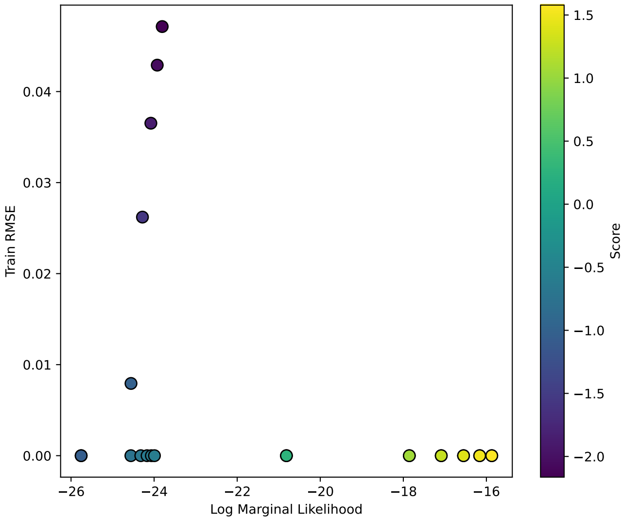
LML vs RMSE (T0)
