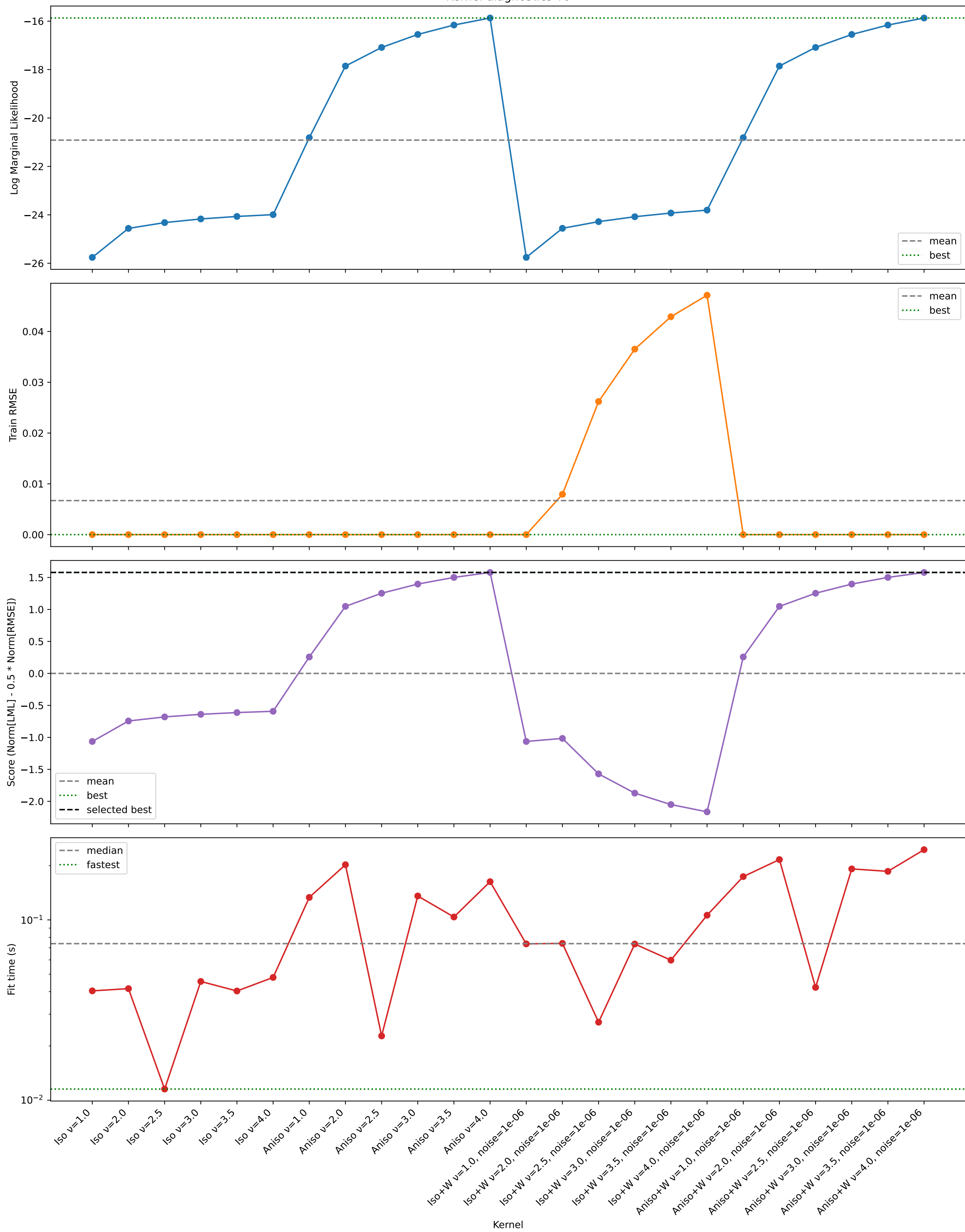
Kernel diagnostics T0
